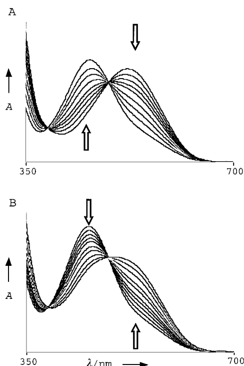
Figure 1. UV/Vis spectra of 2 . A) Addition of 1 to a constant concentration of 2 (180 \mu\text{M} ) results in an increase in the absorbance at 450 nm with a decrease in absorbance at 525 nm. B) Addition of tartrate to a solution containing both 1 and 2 (180 \mu\text{M} each) at a constant concentration causes a decrease in the absorbance at 450 nm and an increase in the absorbance at 525 nm.
